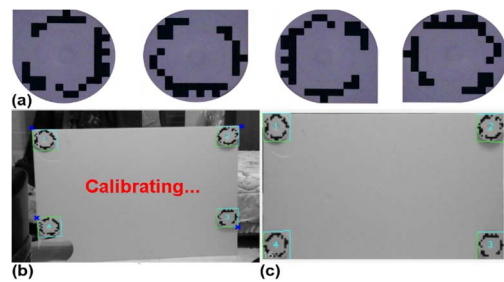
Fig. 8: Automated calibration procedure for easier setup
