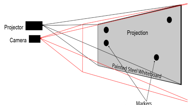
Fig. 1: TangiBoard architectural setup
