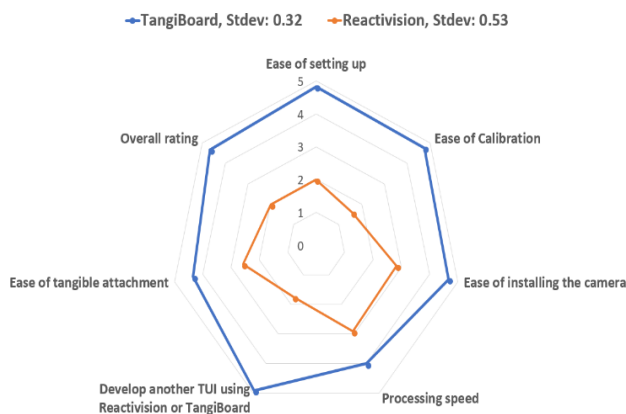
Fig. 9: Comparative results of the determinants evaluated by system designers on both TUI platforms respectively.
